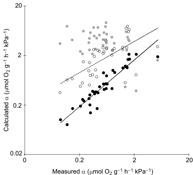
Fig. 4. The measured ( \alpha -method) and calculated (published MR/ P_{crit} ) oxygen supply capacity ( \alpha ). Values are presented in Table S1. The measured \alpha (x-axis) is strongly correlated with that determined as MR/ P_{crit} (y-axis) using reported values (black symbols, y = 1.07x - 0.10 ; Pearson's R = 0.96 , P < 0.001 ). Oxygen supply capacity is significantly correlated with MR ( \alpha = 0.195 \times \text{SMR} + 0.317 ; Pearson's r = 0.98 , P < 0.001 ; open symbols), but not the reported P_{crit} value (Pearson's r = -0.10 , P = 1 ; gray symbols). Data from Behrens and Steffensen, 2007; Birk et al., 2018; Birk et al., 2019; Brill et al., 2015; Burggren et al., 2019a,b; Caposella 2012; Childress, 1975; Childress and Seibel, 1998; Christensen and Colacino 2000; Claireaux and Chabot 2016; Collins et al., 2013; Cowles and Childress, 1995; Crear and Forteach, 2000; Dall 1986; Ern et al., 2016; Fu et al., 2011; Lefevre et al., 2015; Mandic et al., 2020; Negrete and Esbaugh, 2019; Nilsson and Ostlund-Nilsson, 2004; Onthank et al., 2021; Paschke et al., 2010; Reemeyer and Rees, 2019; Rutherford and Thuesen, 2005; Schurmann and Steffensen, 1997; Seibel and Childress, 2000; Slesinger et al., 2019; Snyder et al., 2016; Speers-Roesch, 2012; Staples et al., 2000; Stoffels 2015; Thuy et al., 2010; Tuong et al., 2018; Ultsch et al., 1981; Wishner et al., 2018.
